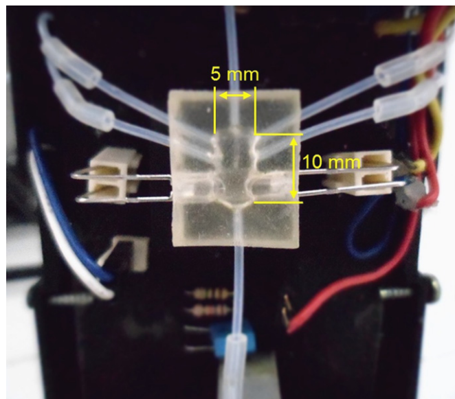
Fig. 1. Photograph of the microfabricated \mu\text{FBA} with its dimensions (mm).
